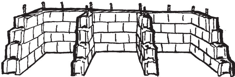
b. Cement block three-bin composting unit.
