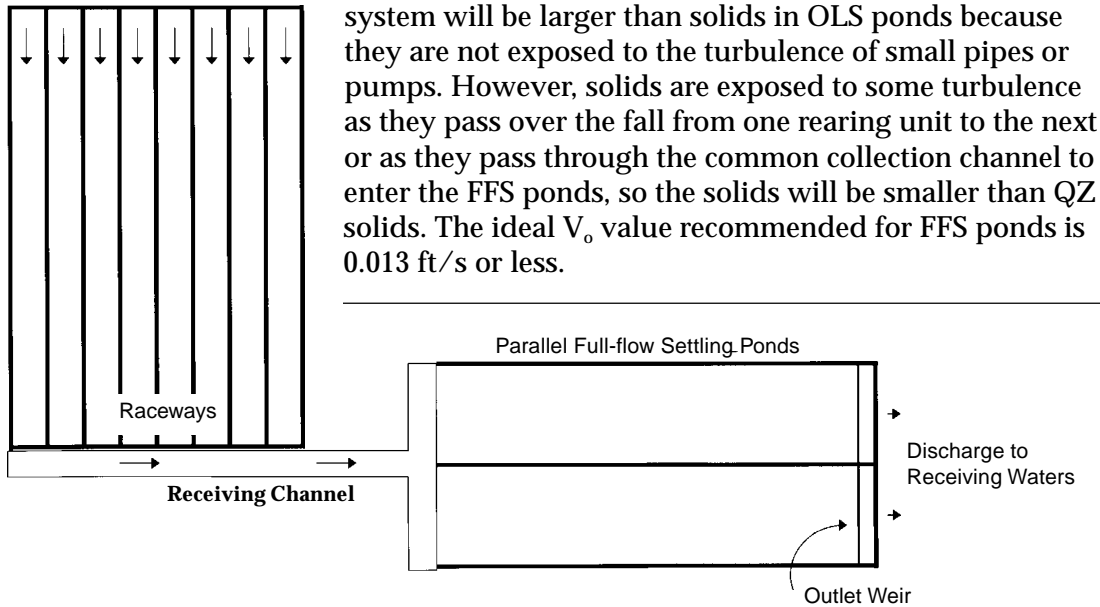
Diagram 7.10: Full-flow settling ponds treat 100% of the flow from the fish farm before it is discharged.
