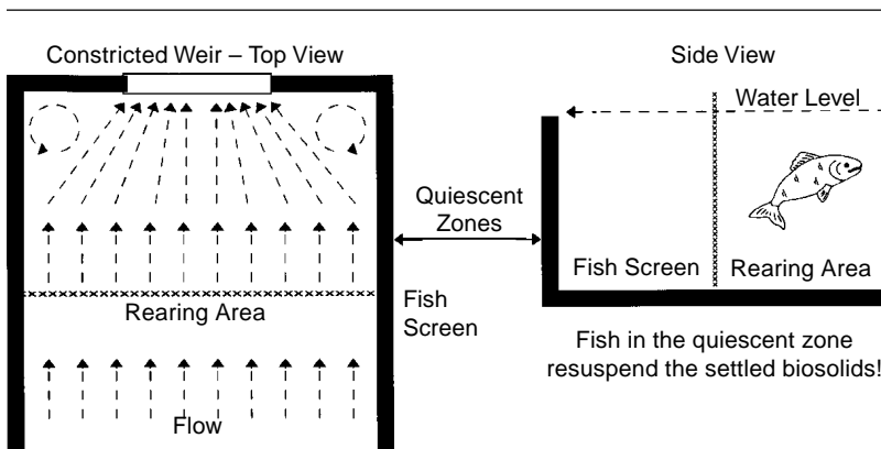
Diagram 7.5: A constricted weir causes turbulence and scouring of settled biosolids. Quiescent zone length should be increased to compensate for the reduced efficiency of the settling zone.
