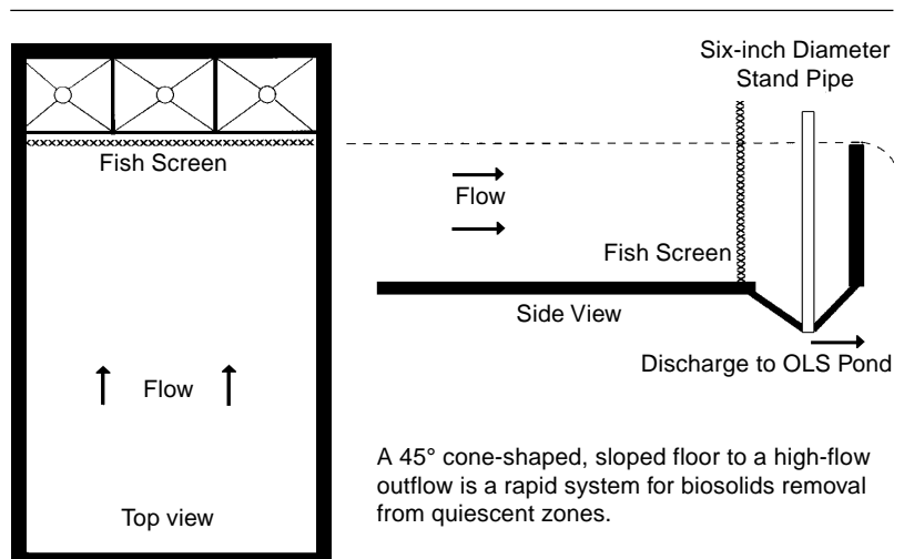
Diagram 7.8: Quiescent zone with a sloped, recessed floor.
