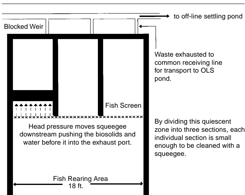
Diagram 7.7: An alternative cleaning method—“subdividing quiescent zones.”
