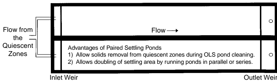
Diagram 7.9a and b: Off-line settling ponds.
