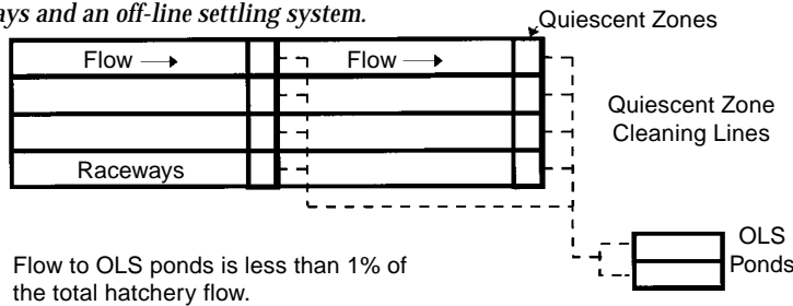
b: Parallel off-line settling ponds.
