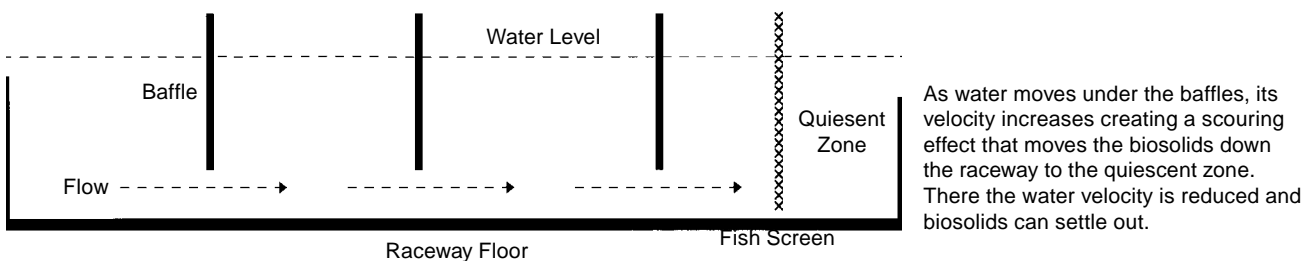
Diagram 7.11: Baffles
