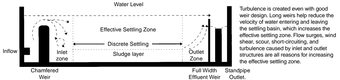
Diagram 7.4: The effective settling zone.
